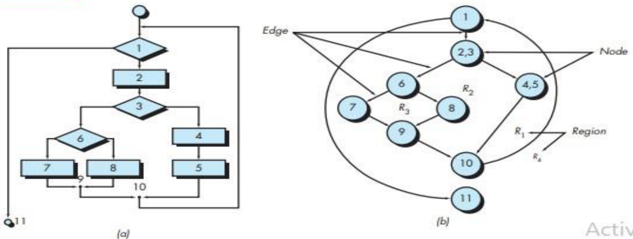
FIGURE 23.2 (a) Flowchart and (b) flow graph
