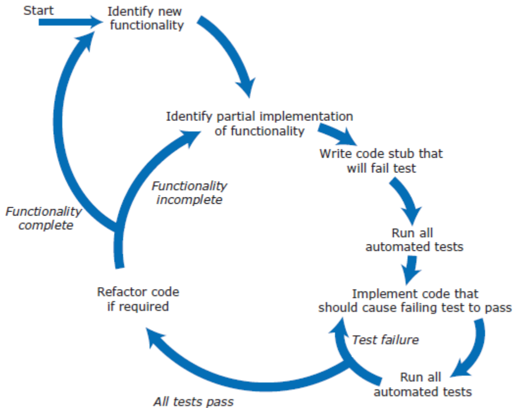
Figure 9.8 Test-driven development
