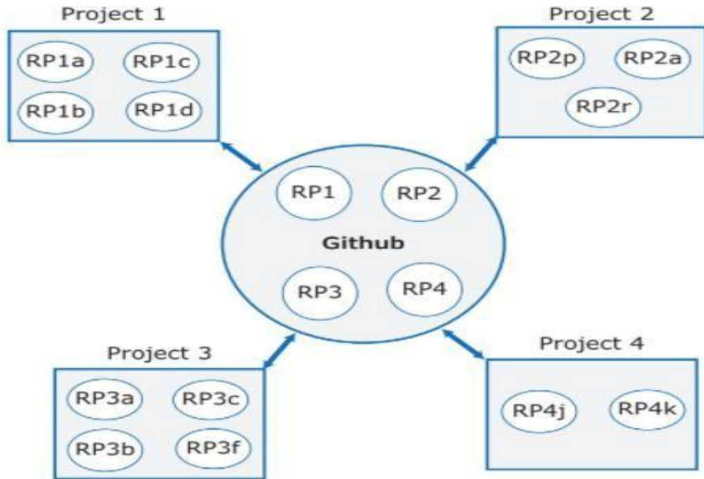
Figure 6 Git repositories
